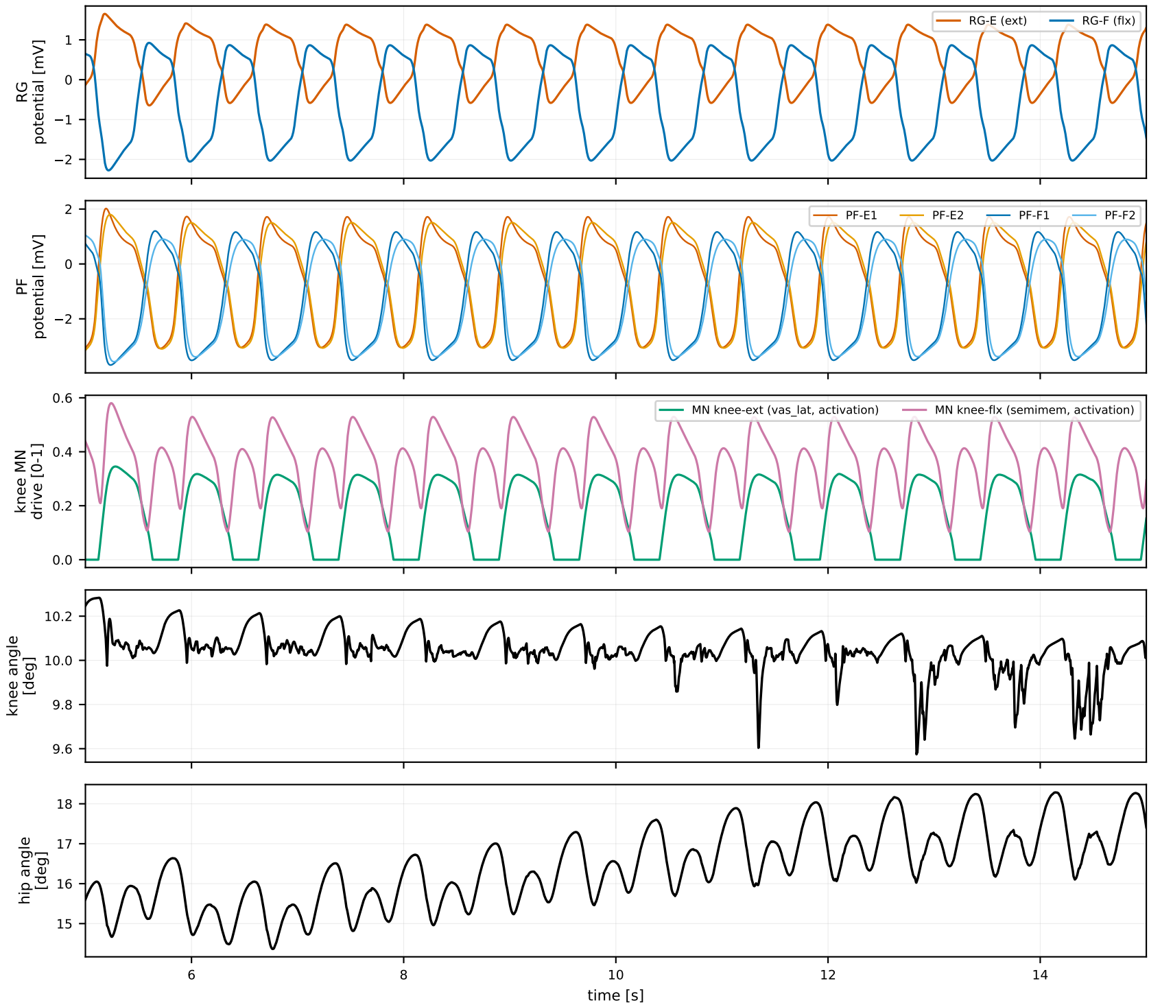
gait2392 spinal SNS - right leg (ground, RoM limits + Renshaw 0.5)
